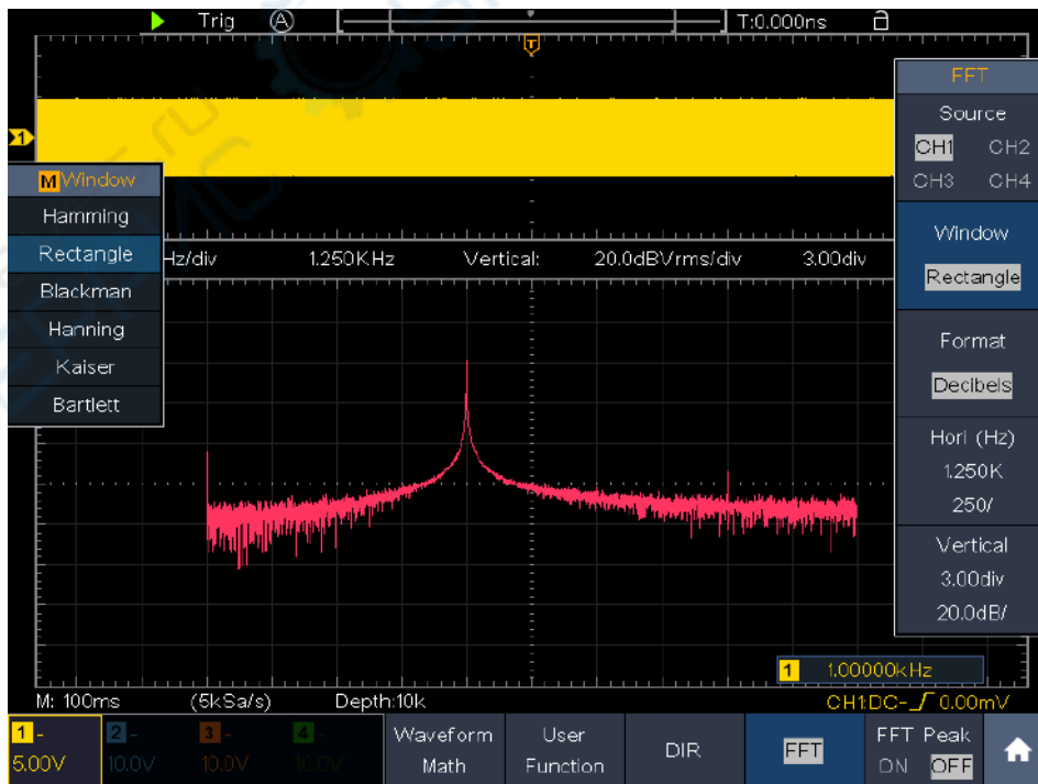
Figure 4-2 Rectangle window
