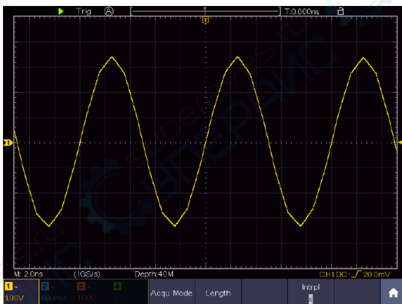
Figure 4-10 Linear interpolation
