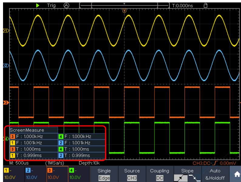
Figure 4-23 Automatic measurement
