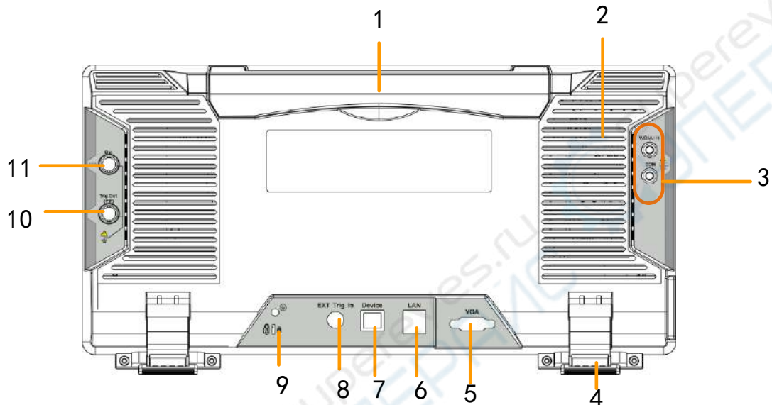
Figure 3-2 Rear Panel
