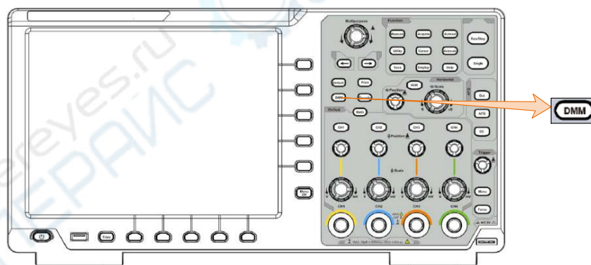
Figure 6-2 Multimeter Button
