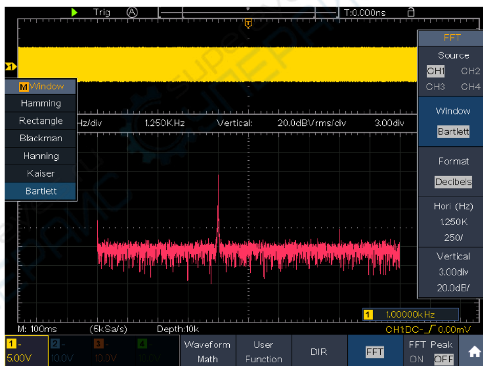
Figure 4-6 Bartlett window
