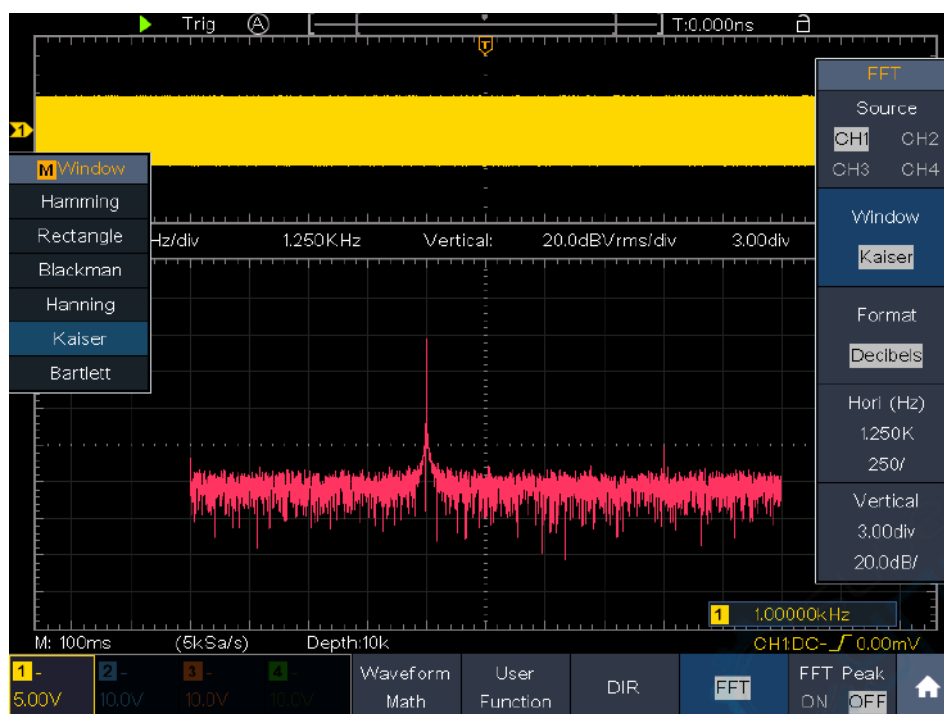
Figure 4-5 Kaiser window
