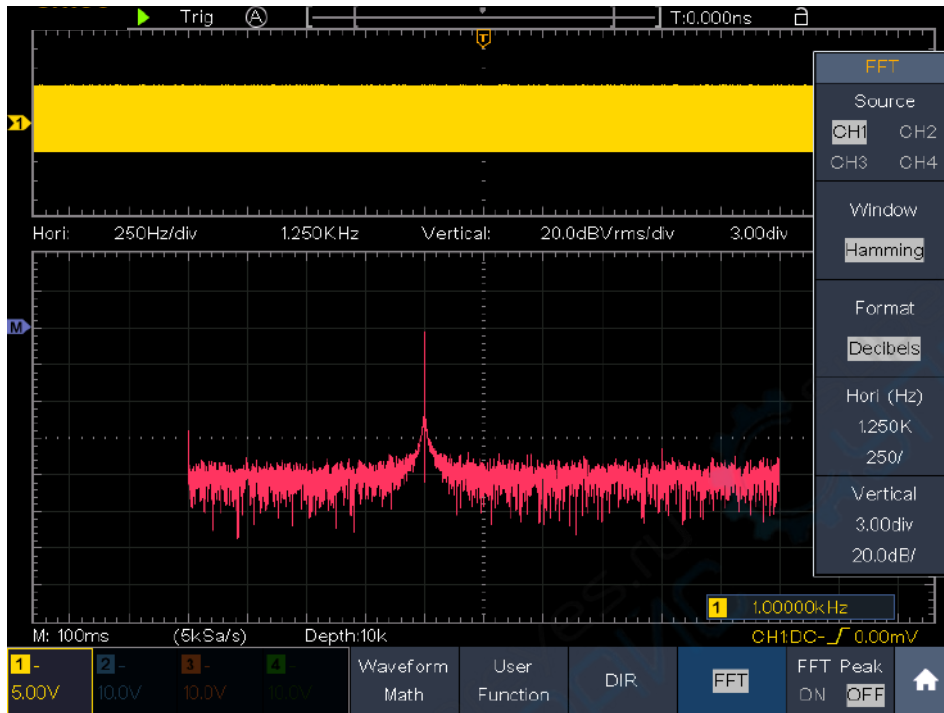
Figure 4-1 Hamming window
