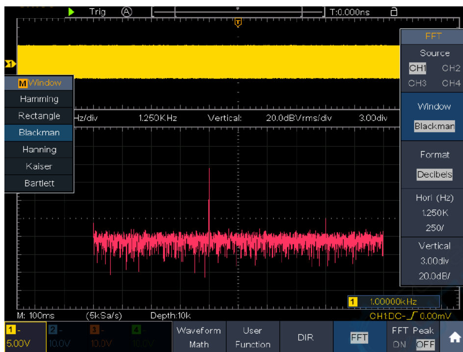
Figure 4-3 Blackman window
